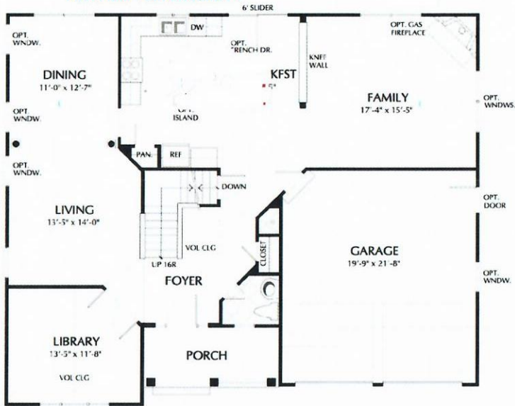
First Floor Plan Elevation 1
